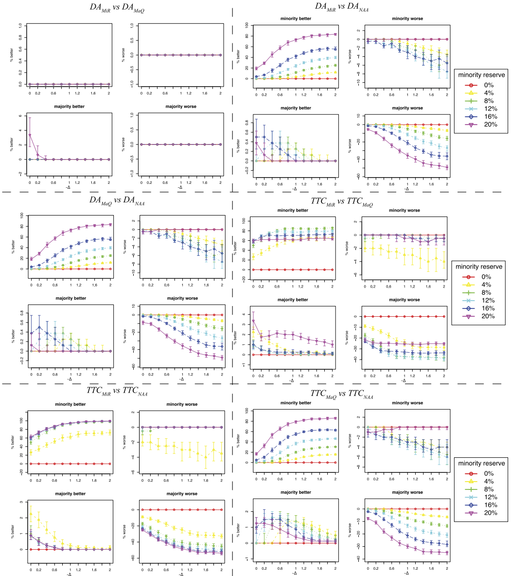
FIGURE S.4. Median percentage of minorities and majorities who are better/worse off under different mechanisms after 100 simulations. The error bars indicate interquartile range. We set the number of students to n = 1,000 , the number of schools to m = 20 , each school size to M = 50 , and the proportion of minority students to r = 20\% . We introduce a new variable, \Delta , which is the average preference of schools toward minority students. We set \alpha = \theta = 0.5 and vary \Delta along with the minority reserve ratio.
