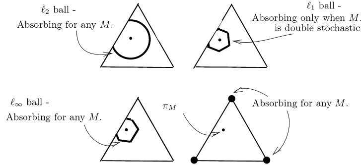
FIGURE 2. Absorbing sets.
