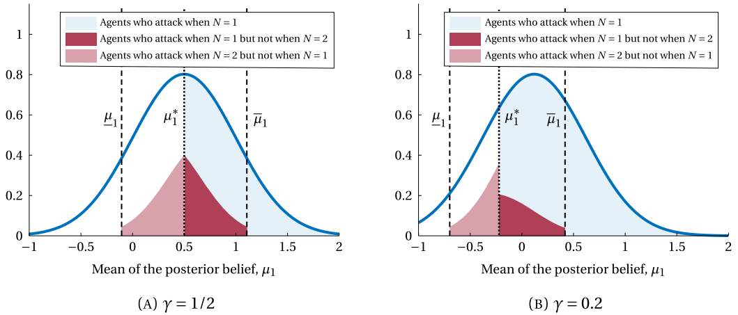
FIGURE 1. The effect of allowing agents to acquire an additional signal when agents have an improper prior. The solid blue line depicts f(\mu_1|\theta_1^*) . The light blue area is equal to the proportion of agents attacking the regime in the model without additional information. The dark red area is equal to the proportion of agents who switch from attacking to not attacking when they can acquire an additional signal. Similarly, the light red area is equal to the proportion of agents who switch from not attacking to attacking when they can acquire an additional signal. Parameters: H - L = 4 , \tau_1 = \tau = 4 , C = 0.025 , R(\theta, p) = \theta + p - 1 .
